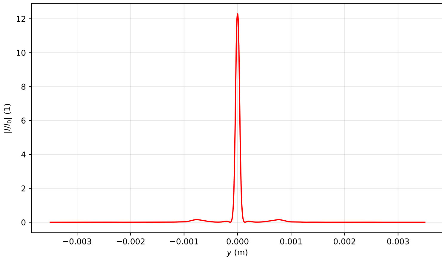
Intensity profile I(x=0, y, z=1.433)/I_0 , P_{in}=8.5P_{cr} , artificial time
